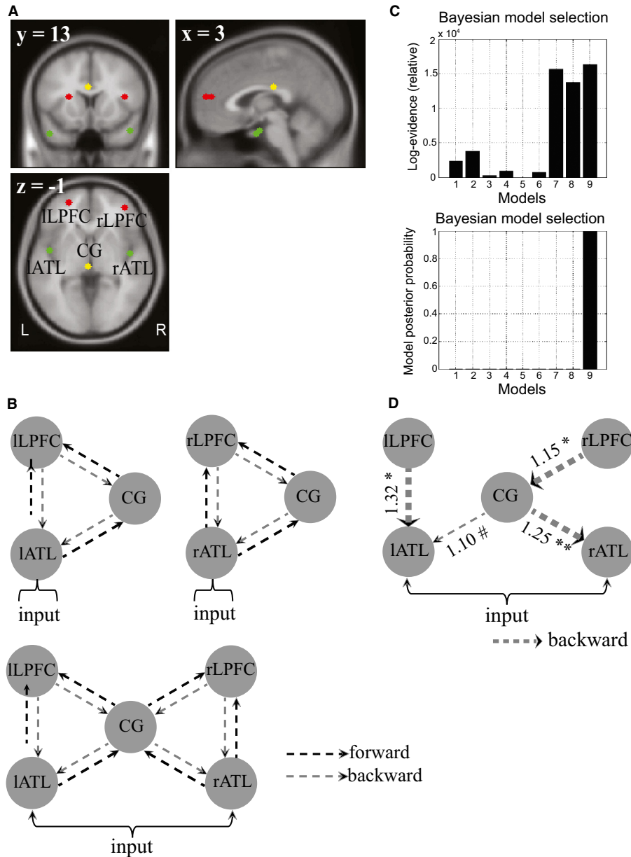
FIG. 6. Source reconstruction and DCM results. (A) Five ROIs in MNI space (in mm): IATL [−46, −4, −32], rATL [46, −8, −28], ILPFC [−24, 54, 14], rLPFC [40, 48, 14] and CG [−2, −24, 26]. (B) Nine candidate DCMs [left-unilateral, right-unilateral or bilateral; forward (F-model), backward (B-model), or both pathways (FB-model)]. (C) Bayesian model selection (BMS) indicated that the bilateral FB model was the optimal one. (D) The effects of reward on connection strength of the optimal model ( ^{\#}P = 0.07 , *P < 0.05 , **P < 0.01 ).
